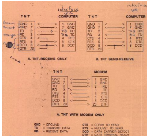
Figure 4/4a. RS-232 Cable Configurations
