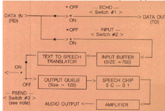
Figure 5 Block Diagram of a TNT with the software controlled switches at their power-up positions
